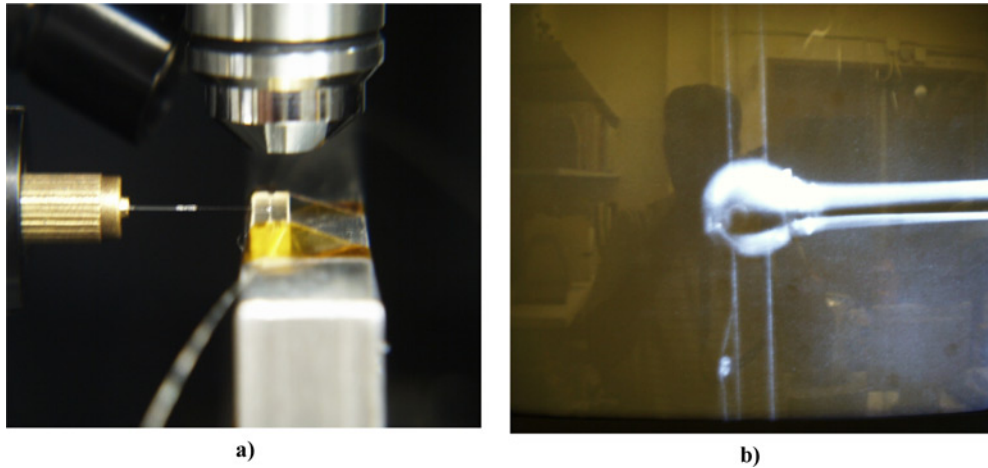
Fig. 9 Microsphere on the top of a half-block coupler: a) setup showing a microsphere on a fiber stem positioned on the coupler; b) microscope image of a microsphere on the top of 125 \mu\text{m} single mode fiber.
