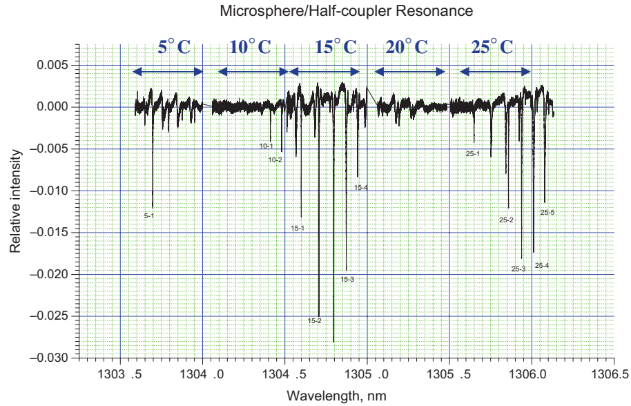
Fig. 11 Resonances over extended range of wavelengths (adopted from [27]).
