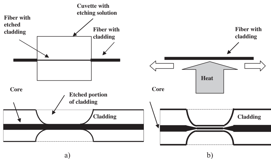
Fig. 7 Thinning of an optical fiber by: a) etching and b) heating and stretching.
