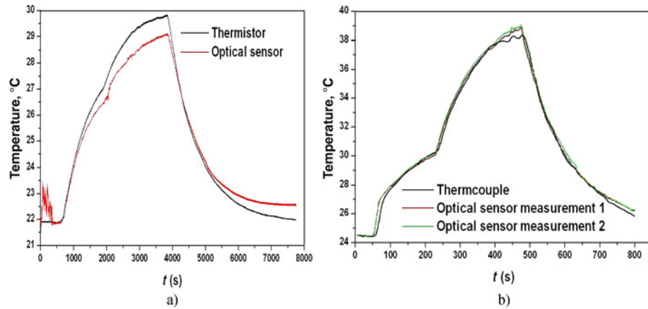
Fig. 13 Temperature measurements in a) water and b) air (from Guan et al. [37]).
