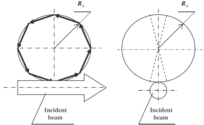
Fig. 4 Schematic explanation of formation of dense resonances in imperfect microspheres.
