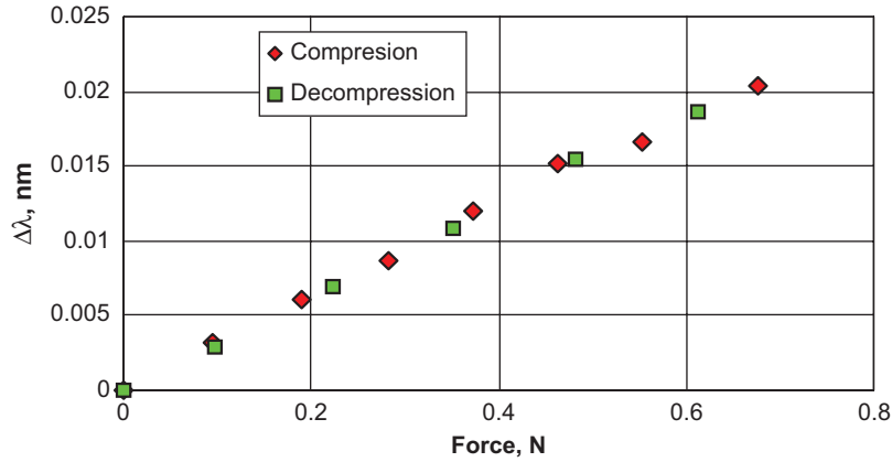
Fig. 15 MDR shift with applied force on a 430 \mu\text{m} -diameter solid silica (from Kozhevnikov et al. [40]).
