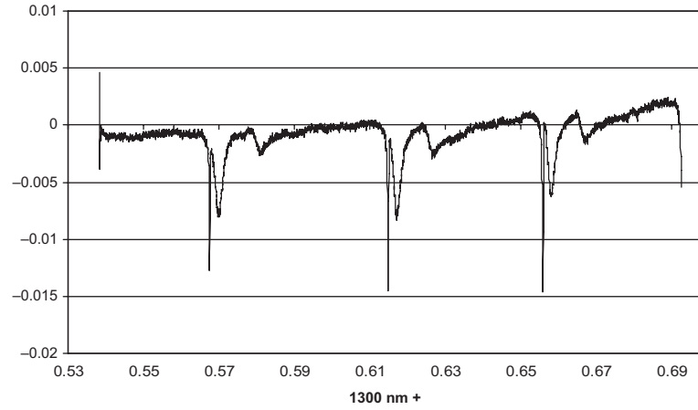
Fig. 3 Resonances in a microsphere with a radius of \sim 200 \mu\text{m} .
