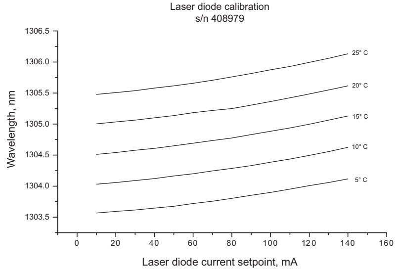
Fig. 10 Laser diode calibration curves at different temperatures (from Adamovsky et al. [27]).
