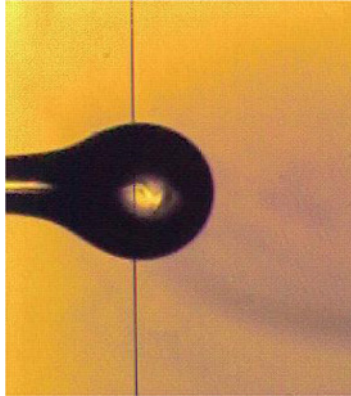
Fig. 8 Microsphere in a close proximity to etched fiber (taken from Guan et al. [37]).
