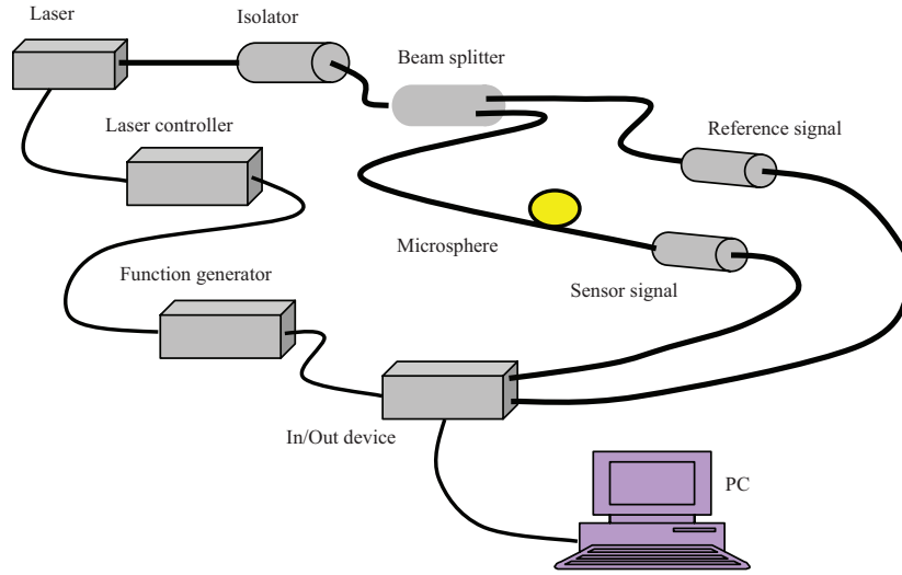
Fig. 12 Schematic of experimental setup (from Das et al. [24].
