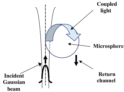
Fig. 5 Schematics of a Gaussian beam coupled into a microsphere.
