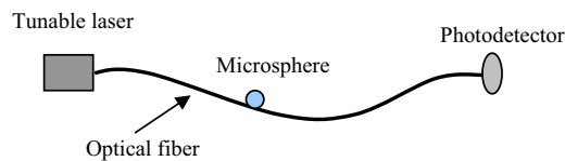
Fig. 1 Interrogation of optical resonances of a microsphere by side-coupled optical fiber.
