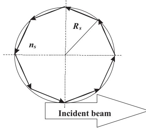
Fig. 2 Principle of MDRs.
