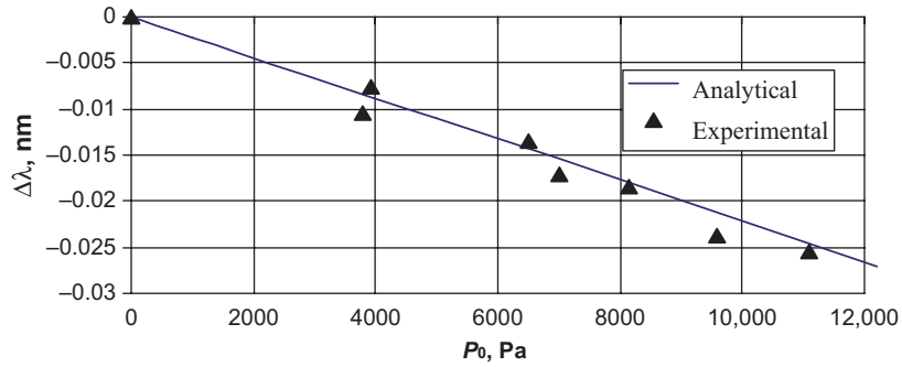
Fig. 16 Pressure tuning of WGM in hollow PMMA sphere with R_S = 500 \mu\text{m} and b/a = 0.95 (from Ioppolo and Ötügen [42]).
