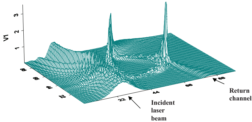
Fig. 6 Computational demonstration of morphology dependent resonances.
